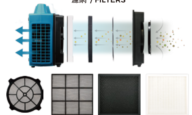
簡便開合設計， 方便用戶快速更換濾網 Tool-free filter changes to replace filter easily.
